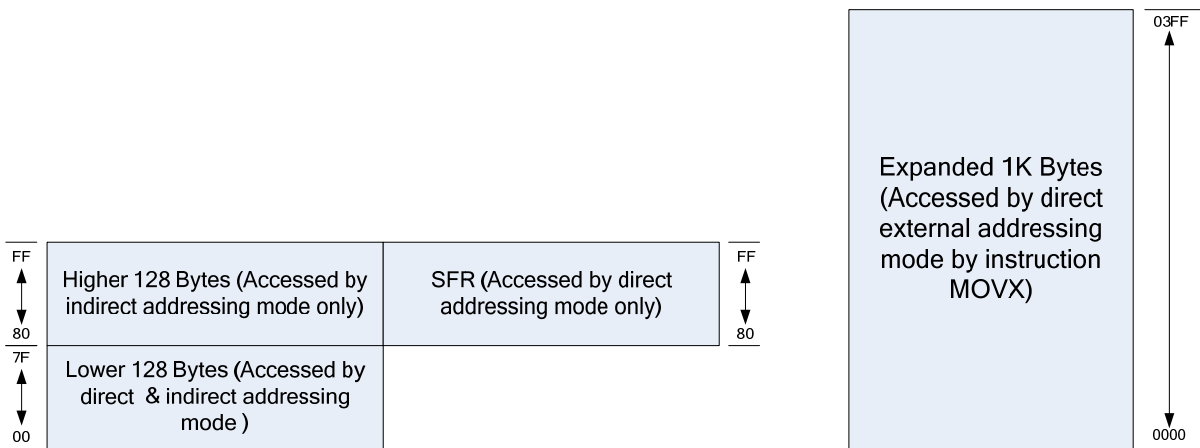
Fig. 3-3: RAM architecture
